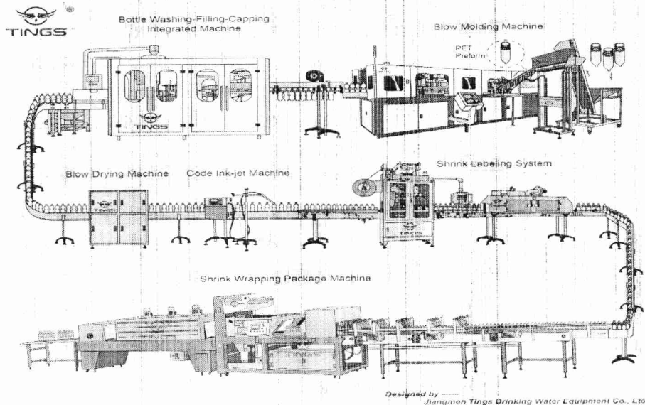
Pic.4 Water bottling line
