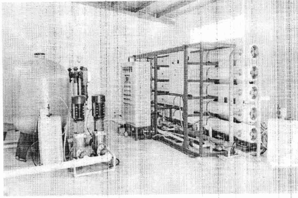
Pic.2 Reverse Osmosis Cleaning Equipment
